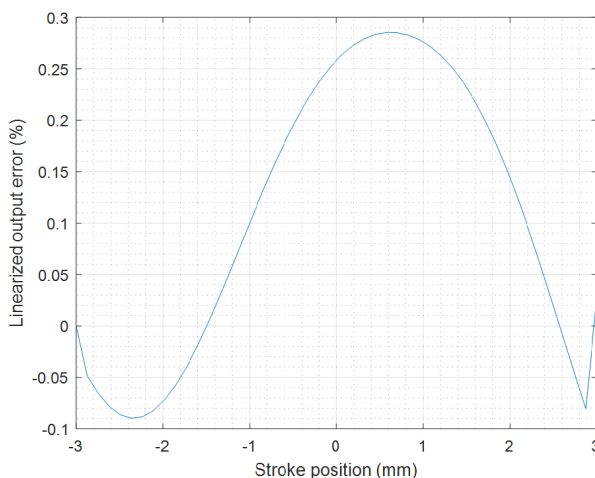
Figure 13: Linearization error as a percent over the full range, smoothing applied
