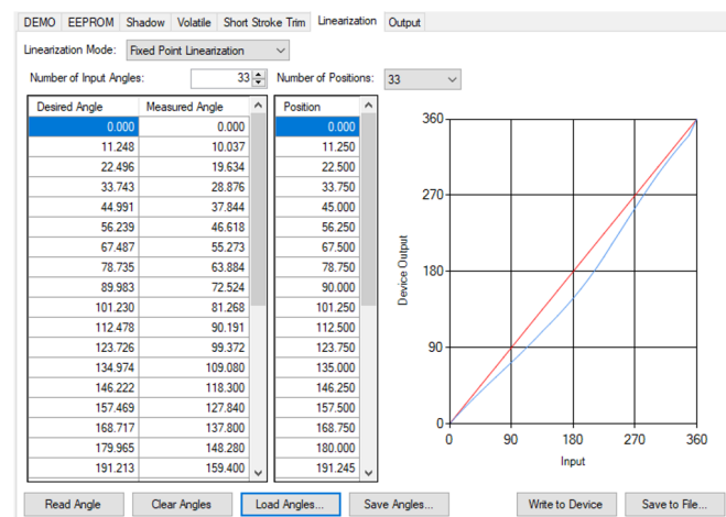
Figure 11: Linearization Tab with sensed values (as angles) recorded
