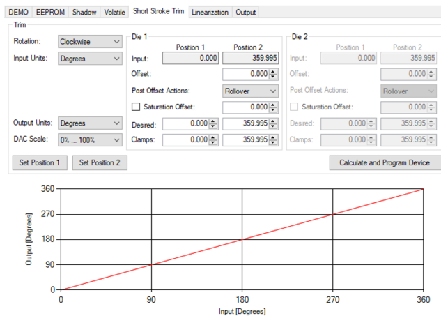
Figure 9: The Short-Stroke tab
