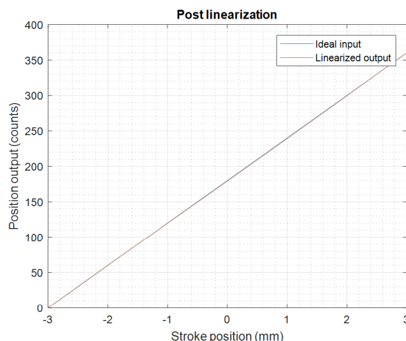
Figure 12: Resulting output after linearization.
